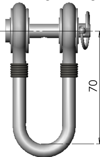
Manille textile / loop shackle Poids/weight : 307g
